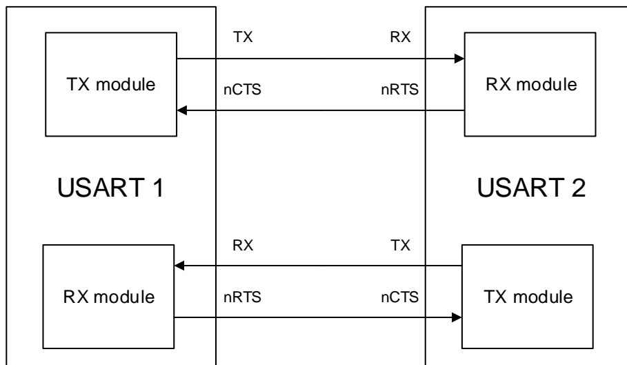
Figure 19-7. Hardware flow control between two USARTs
