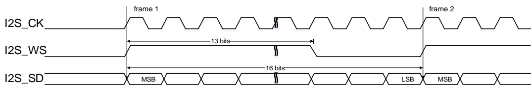
Figure 21-43. PCM standard long frame synchronization mode timing diagram (DTLEN=00, CHLEN=0, CKPL=0)
