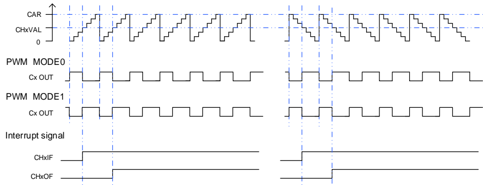
Figure 18-53. EAPWM timechart
