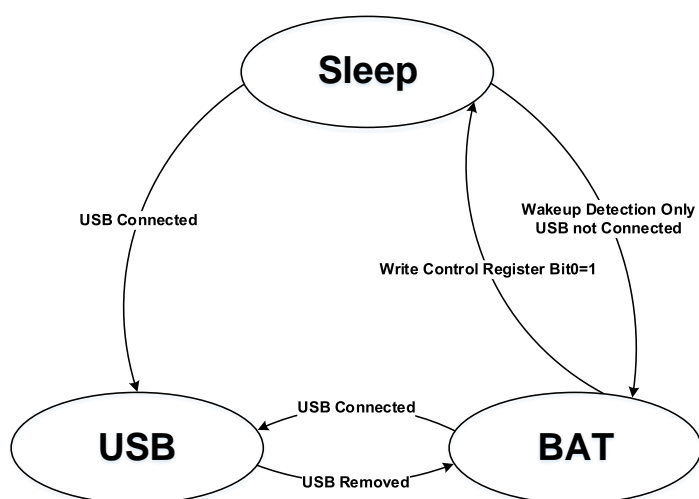
Figure 5-1 Operation modes
