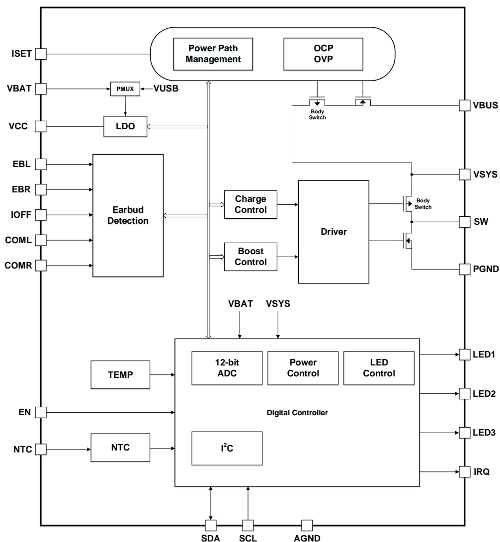
Figure 4-1 Block diagram for GD30WS8855x
