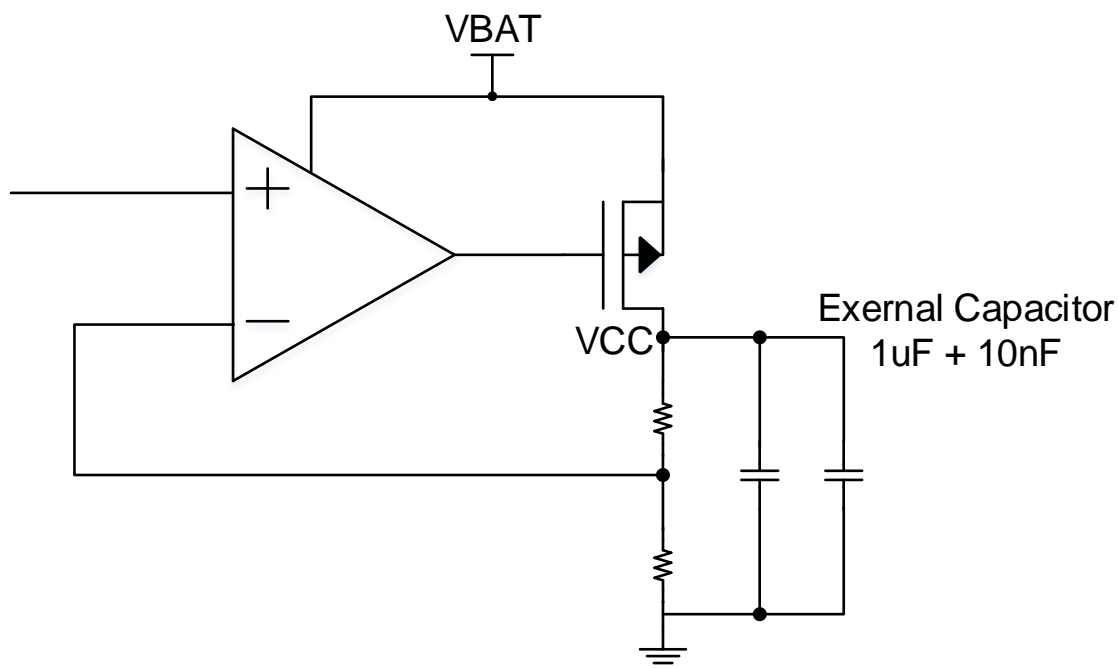
Figure 5-4 The principle diagram for LDO
